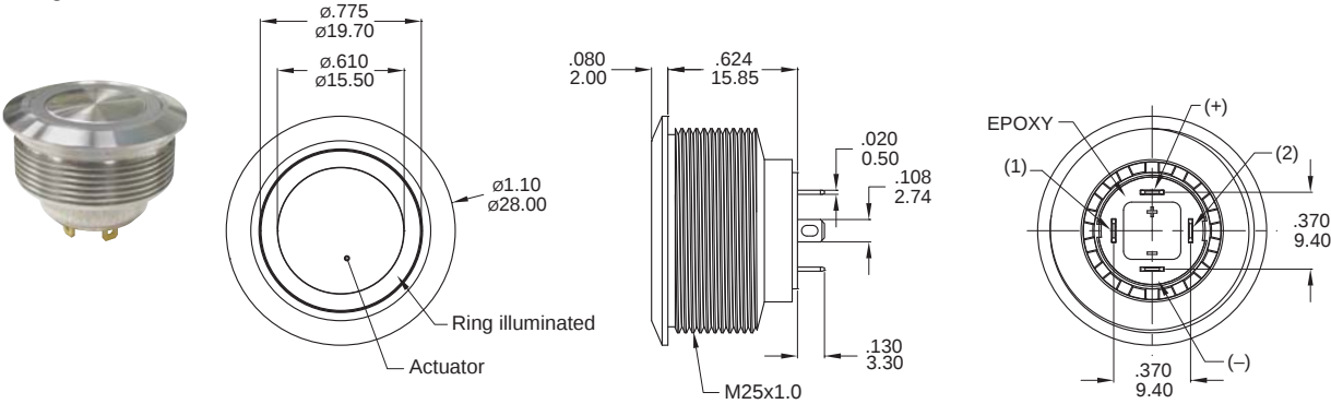
Part No. Shown : MPS25-A02FE-□-JR-□V
