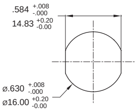
PANEL CUTOUT
