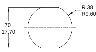
PANEL CUTOUT
